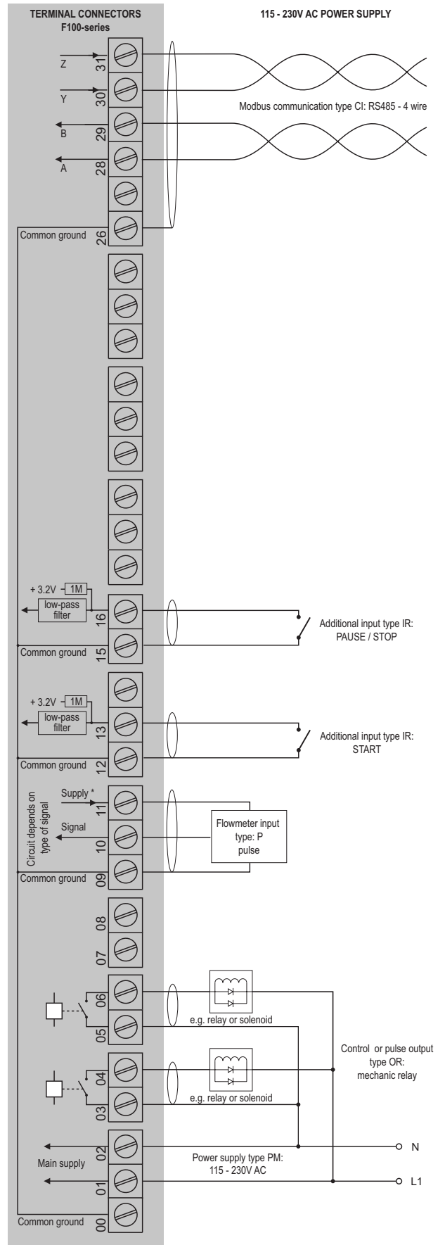
Configuration example F130-P-CI-OR-PM-XX-ZX
